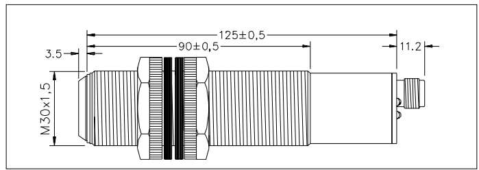
Dimensions/Abmessungen/Dimensions
